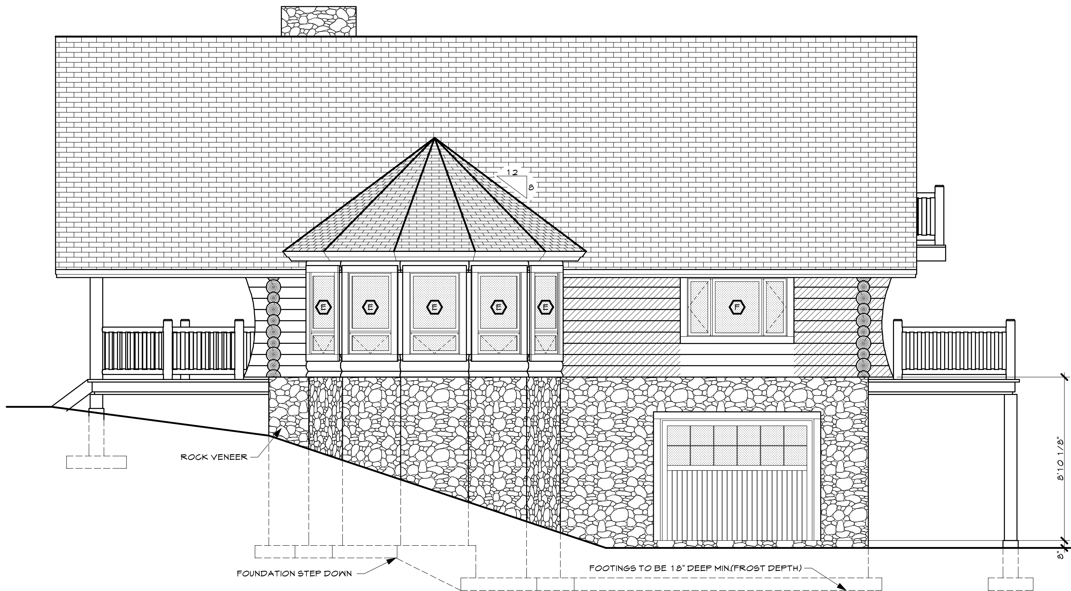
SOUTHEAST ELEVATION 1/4" = 1'-0"
